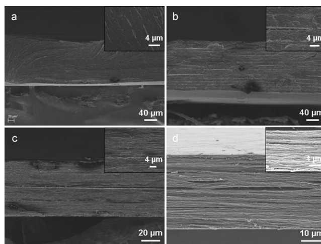
Figure 4. Cross-sectional SEM images of different films. a) Pure chitosan film (4 wt.% chitosan solution, spin coating at 1000 rpm). b) Co-Al-CO 3 -chitosan hybrid film (4 wt.% chitosan solution, spin coating at 1000 rpm). c) Alternative Cu-NO 3 -chitosan-Co-Al-CO 3 -chitosan hybrid film (3 wt.% chitosan solution, spin coating at 1000 rpm). d) Co-assembly 2D structure of V Cu-NO 3 /V Co-Al-CO 3 = 3:1-chitosan hybrid film (3 wt.% chitosan solution, spin coating at 1000 rpm). The inset images are magnifications.
